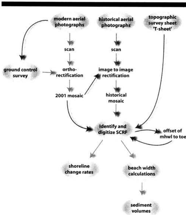
Figure 3. Photogrammetry procedures.
